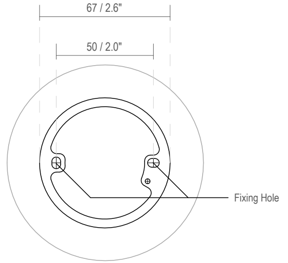
Fixing Dimensions
