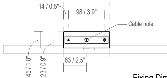
Fixing Dimensions
