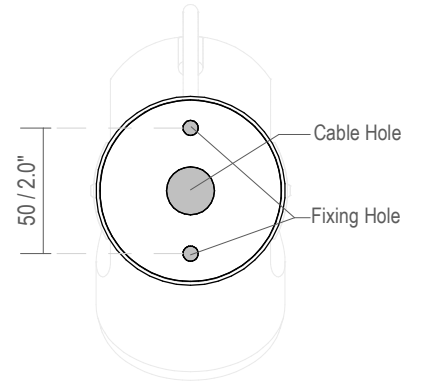
Fixing Dimensions
