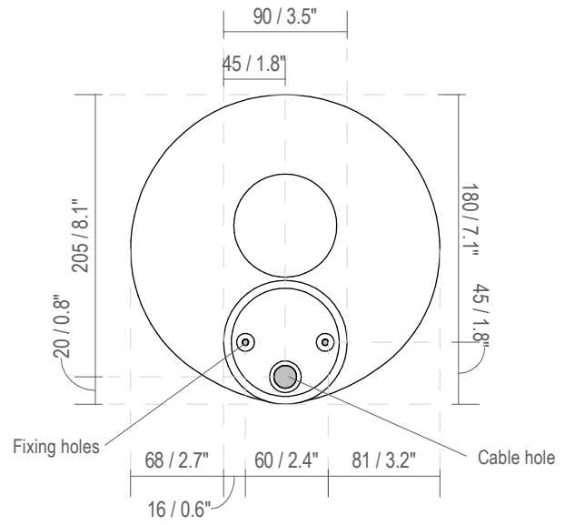
Fixing Dimensions
