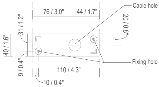
Fixing Dimensions
