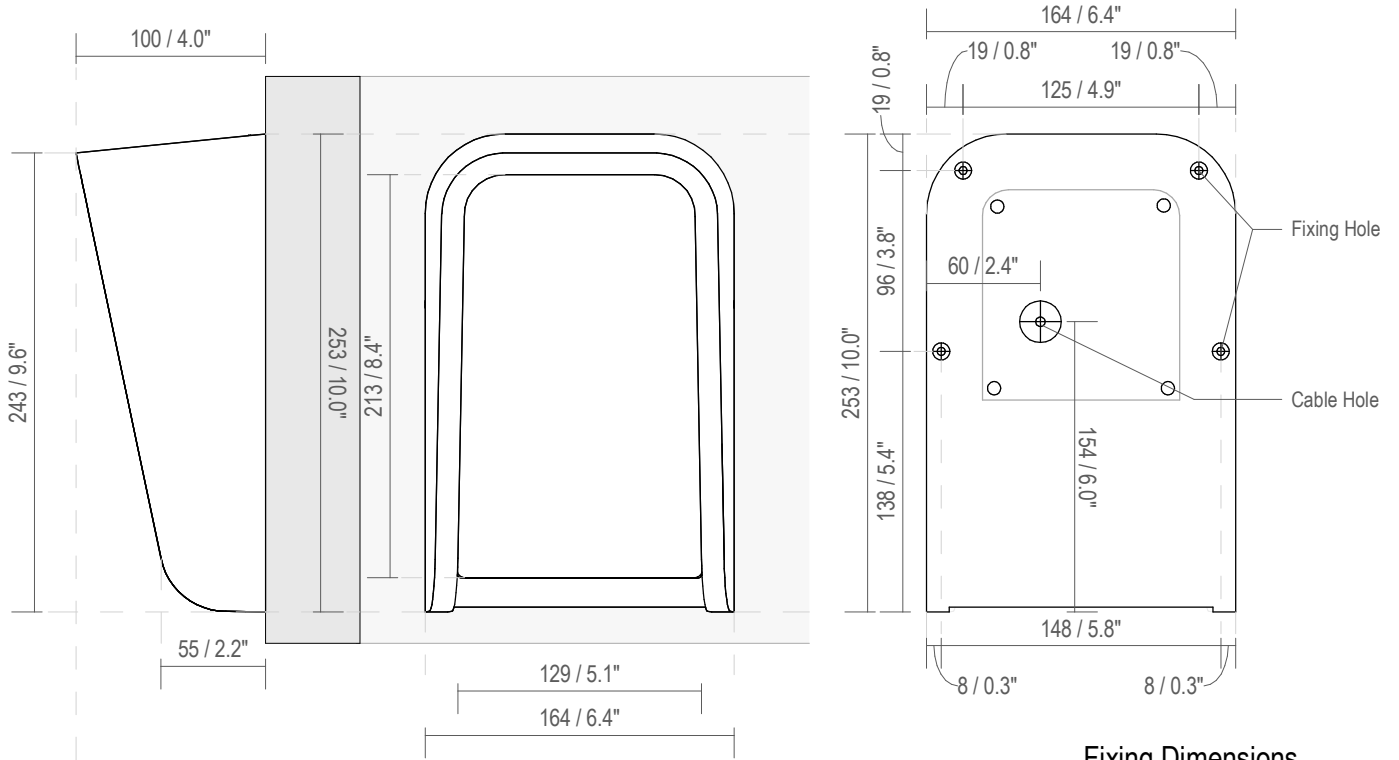
Fixing Dimensions
