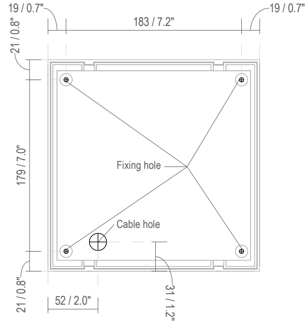
Fixing Dimensions
