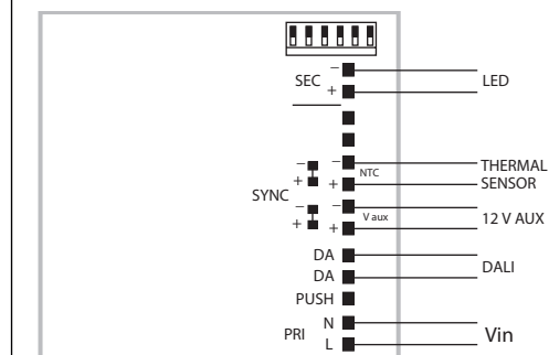
DALI diagram
