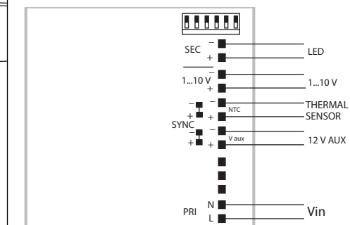
1...10 V diagram
