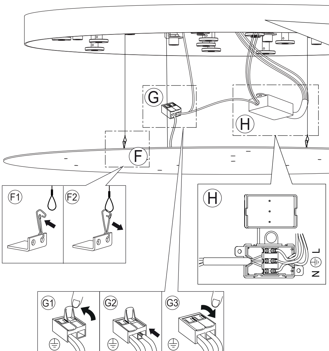
PUSH diagram
