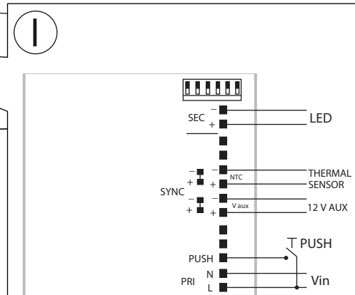
PUSH diagram
